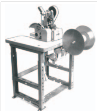
AVAILABLE AS A COMPLETE ASSEMBLED UNIT with HEAVY DUTY STEEL STAND, FORMICA-TYPE TABLE TOP AND 110 VAC MOTOR. Also Available with 220v. 3-phase motor
